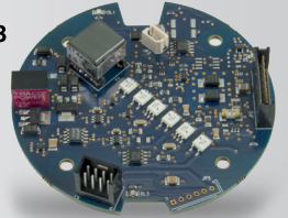
Intrinsically safe PCB & galvanic isolation
